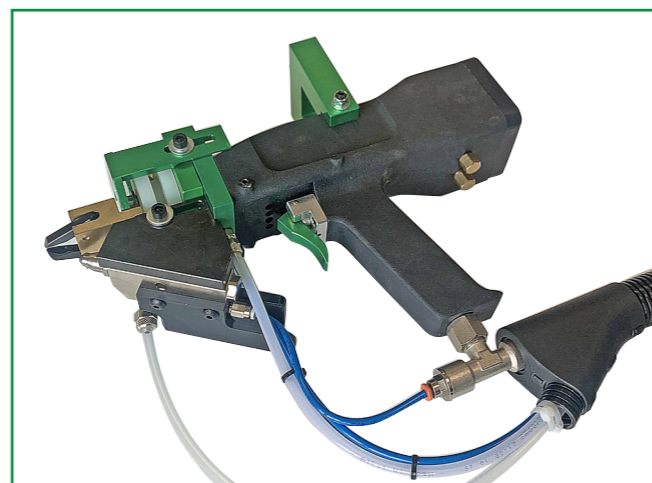
Pistola colla e spine/Gun for glue and dowels
